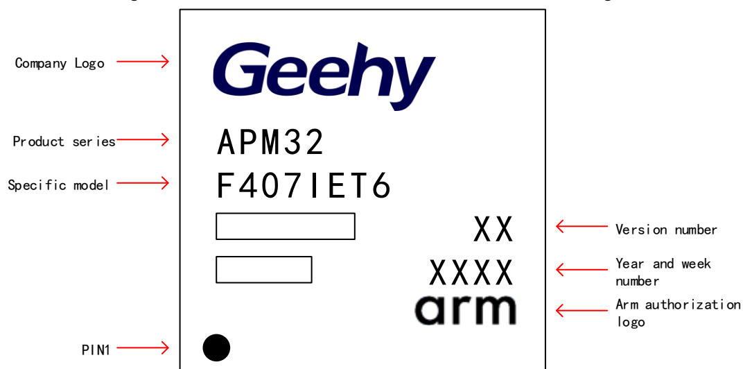
Figure 19 LQFP176 -176 Pins, 24 x24mm Schematic Diagram
