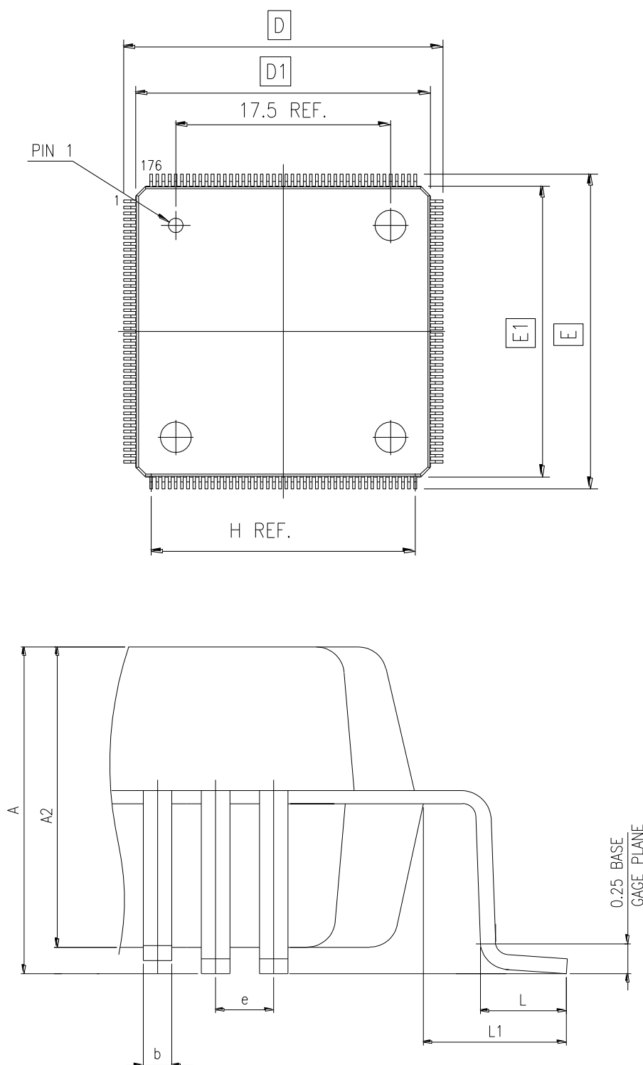
Figure 17 LQFP176 Package Diagram
